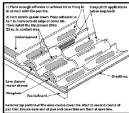
Two Piece Barrel - High Profile Tile
